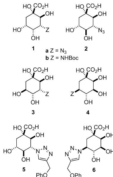
Figure 1. Cyclic \gamma -azido and \gamma -amino acids and triazole derivatives.
