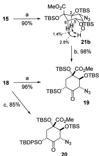
Scheme 7. Reagents and conditions: (a) TBSOTf, Py, DCM, 0 °C → r.t.; (b) (i) DMSO, TFAA, DCM, -60 °C, (ii) Et 3 N, -60 °C → r.t.; (c) TBDPSCl, Im, DMF, 0 °C → r.t.
