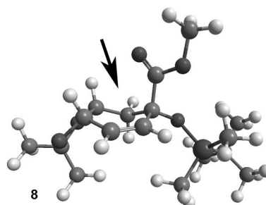
Figure 2. Minimum-energy conformation of cyclohexene 8 obtained by molecular modelling calculations (Gaussian 03W). [8,9]
