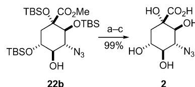
Scheme 8. Reagents and conditions: (a) TFA (aq., 50%), 70 °C; (b) LiOH, r.t.; (c) Amberlite IR-120 (H + ), r.t.
