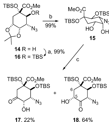
Scheme 6. Reagents and conditions: (a) TBSOTf, Py, DCM, 0 °C \rightarrow r.t.; (b) \text{AcOH} (aq., 80%), 65 °C; (c) (i) \text{Bu}_2\text{SnO} , PhMe, \Delta , (ii) NBS, \text{CHCl}_3 , r.t.
