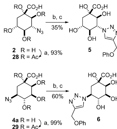
Scheme 12. Reagents and conditions: (a) Ac 2 O, Py, 0 °C \rightarrow r.t.; (b) PhOCH 2 C \equiv CH, sodium ascorbate, t BuOH/H 2 O, CuSO 4 , r.t.; (c) (i) LiOH, r.t., (ii) Amberlite IR-120 (H + ), r.t.
