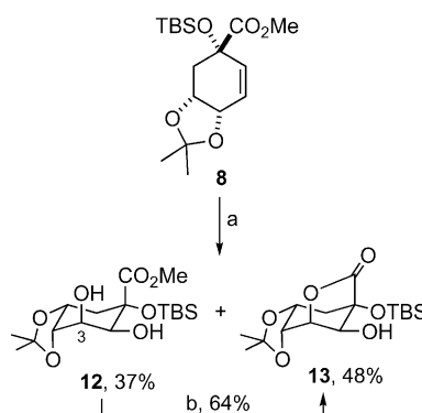
Scheme 3. Reagents and conditions: (a) \text{OsO}_4 (cat), NMO, dioxane/ \text{H}_2\text{O} , r.t.; (b) NaH, THF, 0\text{ }^\circ\text{C} .
