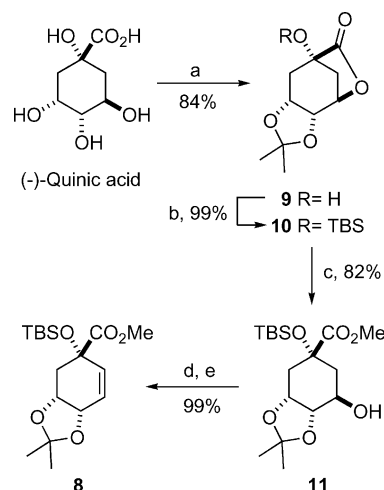
Scheme 2. Reagents and conditions: (a) \text{Me}_2\text{C}(\text{OMe})_2 , \text{HC}(\text{OMe})_3 , acetone, p -TsOH (cat.), \Delta ; (b) TBSOTf, Py, DCM, 0\text{ }^\circ\text{C} \rightarrow \text{r.t.} ; (c) KCN, MeOH, r.t.; (d) \text{Trf}_2\text{O} , Py, DCM, 0\text{ }^\circ\text{C} ; (e) DBU, \text{CHCl}_3 , \Delta .
