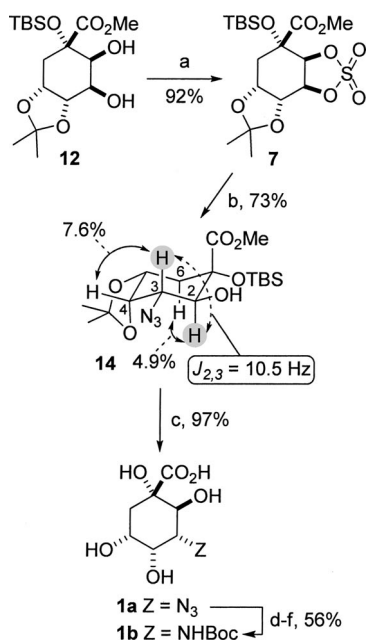
Scheme 4. Reagents and conditions: (a) (i) \text{SOCl}_2 , \text{Et}_3\text{N} , DCM, r.t., (ii) \text{RuCl}_3 \cdot 3\text{H}_2\text{O} (cat.), \text{NaIO}_4 , \text{H}_2\text{O} , \text{CCl}_4 , \text{CH}_3\text{CN} , r.t.; (b) (i) \text{NaN}_3 , 15-crown-5 ether, DMF, 90 °C, (ii) \text{H}_2\text{SO}_4 (aq., 70%), THF, 50 °C; (c) (i) TFA (aq., 50%), 70 °C, (ii) \text{LiOH} , r.t., (iii) Amberlite IR-120 ( \text{H}^+ ), r.t.; (d) \text{Ac}_2\text{O} , Py, 0 °C to r.t.; (e) \text{H}_2 , \text{PtO}_2 (cat.), \text{Boc}_2\text{O} , THF, r.t.; (f) (i) \text{LiOH} , r.t.; (ii) Amberlite IR-120 ( \text{H}^+ ), r.t.
