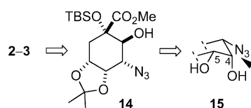
Scheme 5. Strategy for the synthesis of derivatives 2–3 .
