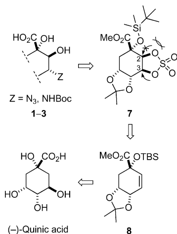
Scheme 1. Strategy for the synthesis of derivatives 1–3 .
